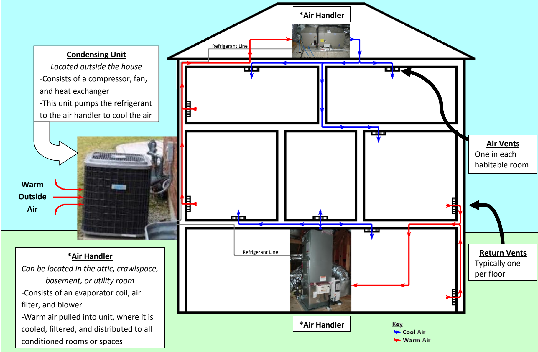
The above diagram shows one air handler in the attic and one in a basement (for the sake of showing the different options). Typically there would be one unit in one location or the other. Multi-zone systems could have multiple air handlers in different locations. In those cases, there would be one condensing unit for each air handler.
